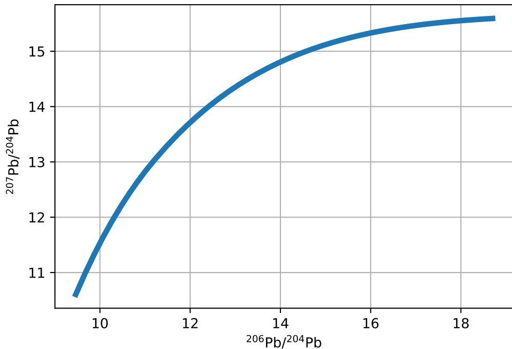
Stacey and Kramers (1975) Common Lead Model
